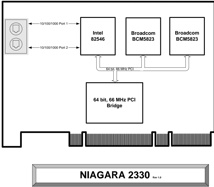
Figure 1 Block diagram
